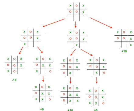
https://www.geeksforgeeks.org/minimax-algorithm-in-game-theory-set-3-tic-tac-toe-ai-finding-optimal-move/
