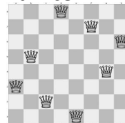
https://www.puzzleprime.com/brain-teasers/deduction/eight-queens-puzzle/
